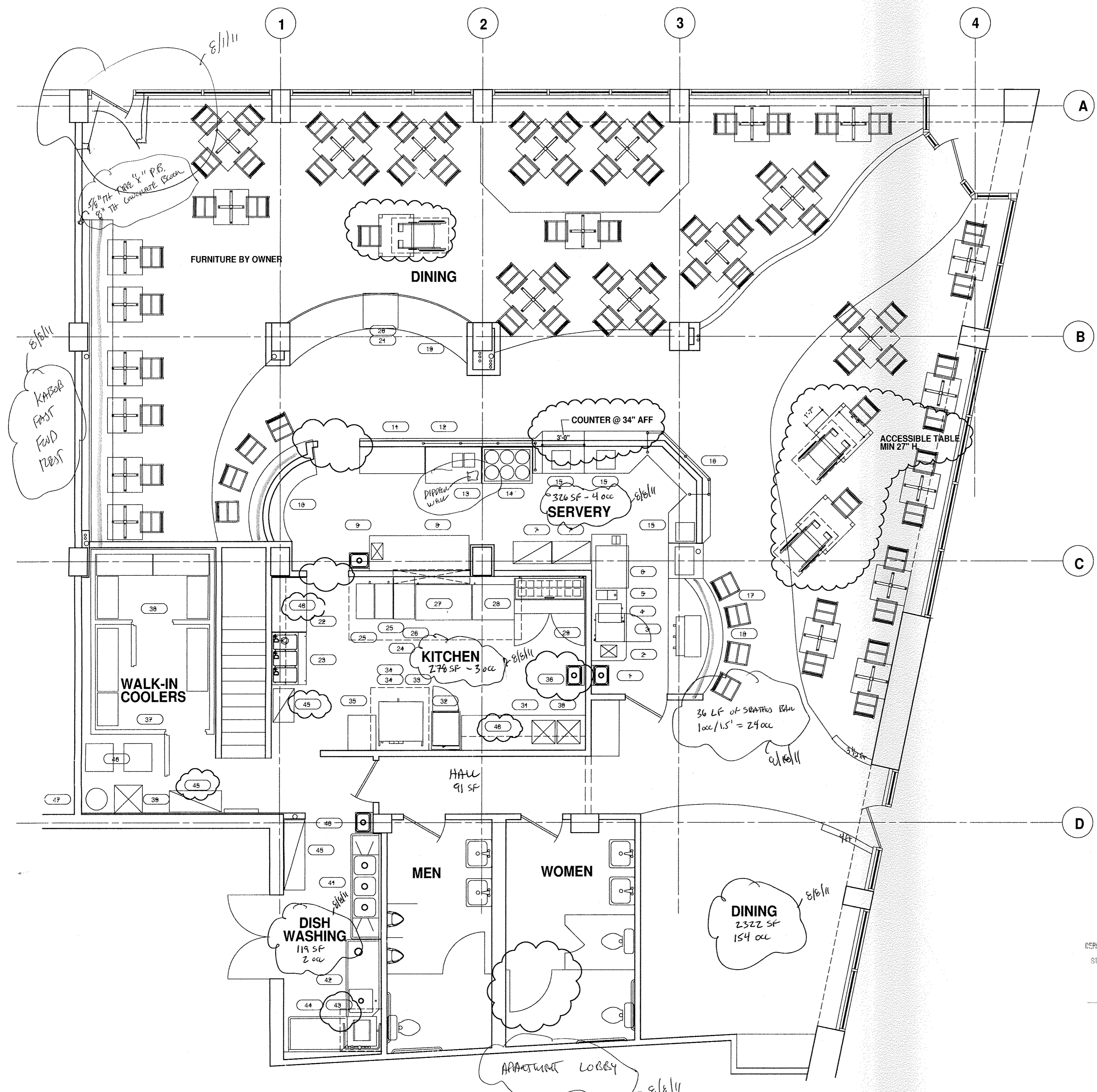
EQUIPMENT PLAN SCALE: 1/4" = 1'-0"
